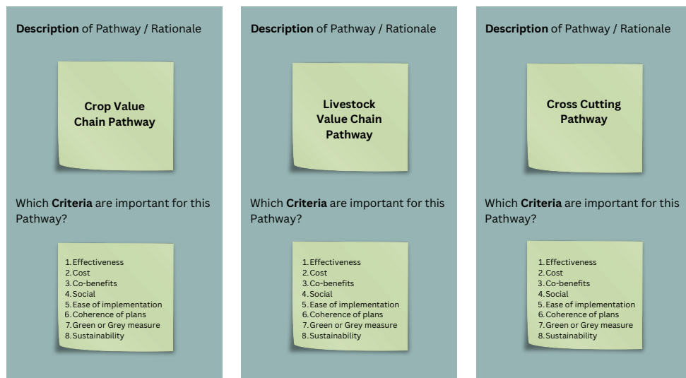
Figure 39: Pathway names and criteria suggestions in the Webinar for the Eastern Province
