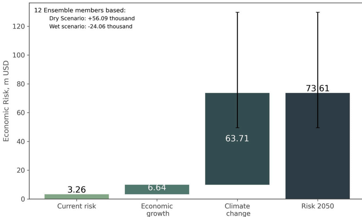
Figure 14: Average annual cattle losses in USD due to droughts today and for different climate change scenarios (RCP 4.5 top and RCP 8.5 bottom) in the future (year 2050).
