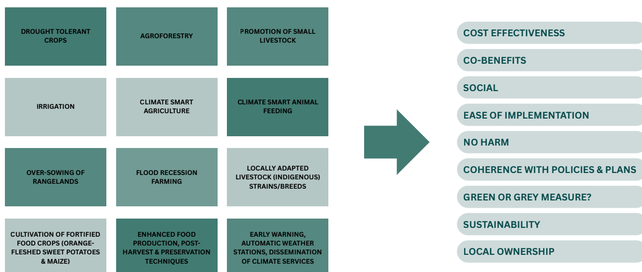
Figure 38: Long list of measures and criteria
