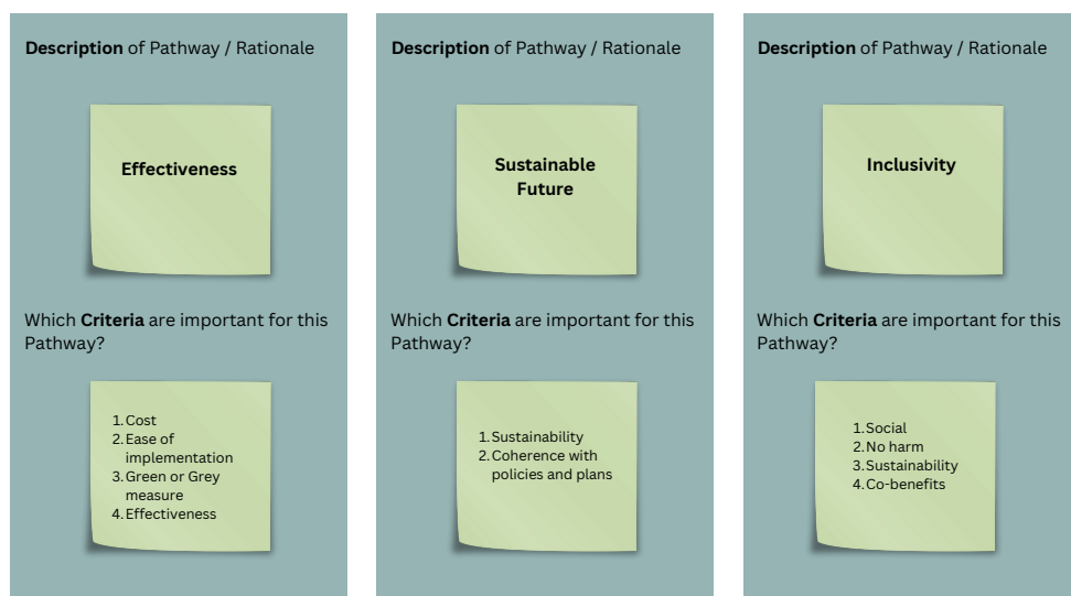
Figure 40: Pathway names and criteria suggestions in the Webinar for the Southern Province
