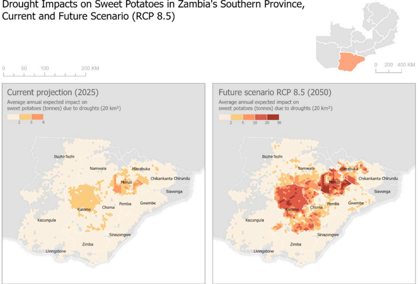
Figure 10: Drought impacts on sweet potato production for current and future (2050, RCP 8.5) scenarios.
