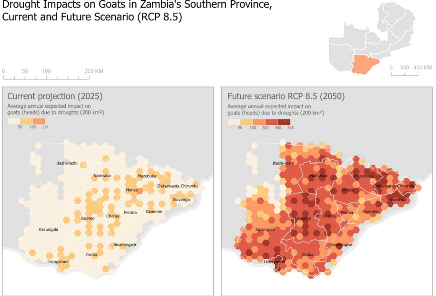
Figure 15: Drought impacts on goat population for current and future (2050, RCP 8.5) scenarios.
