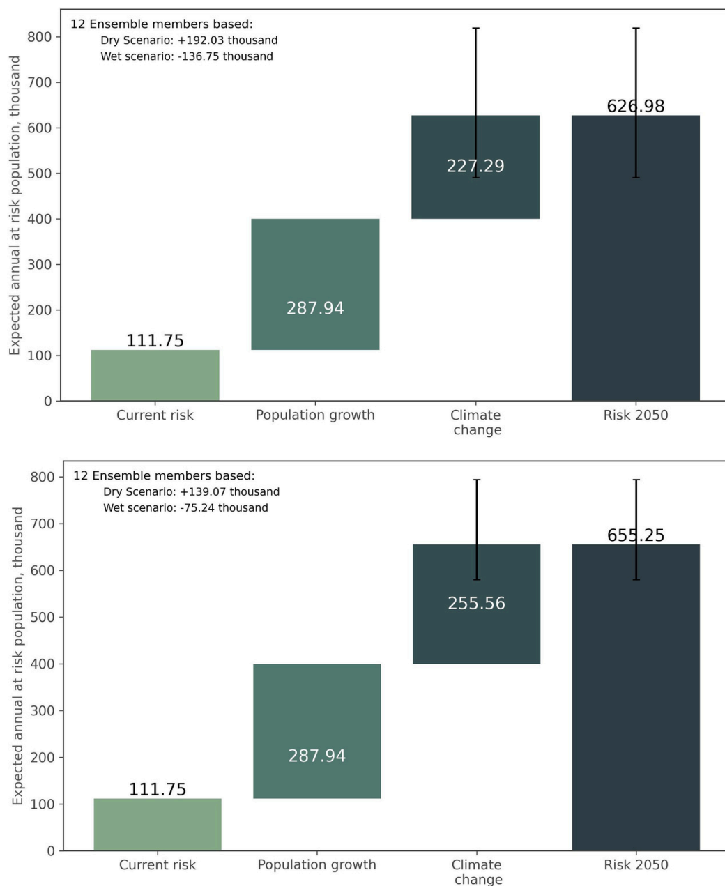
Figure 18: Average Annual number of People facing food insecurity due to droughts today and for different climate change scenarios (RCP 4.5 top and RCP 8.5 bottom) in the future (year 2050).
