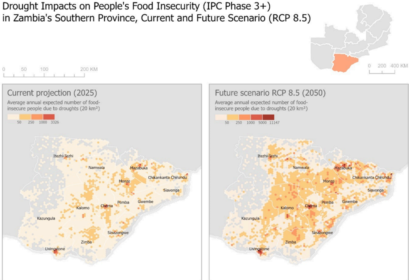
Figure 17: Drought impacts on people for current and future (2050, RCP 8.5) scenarios.
