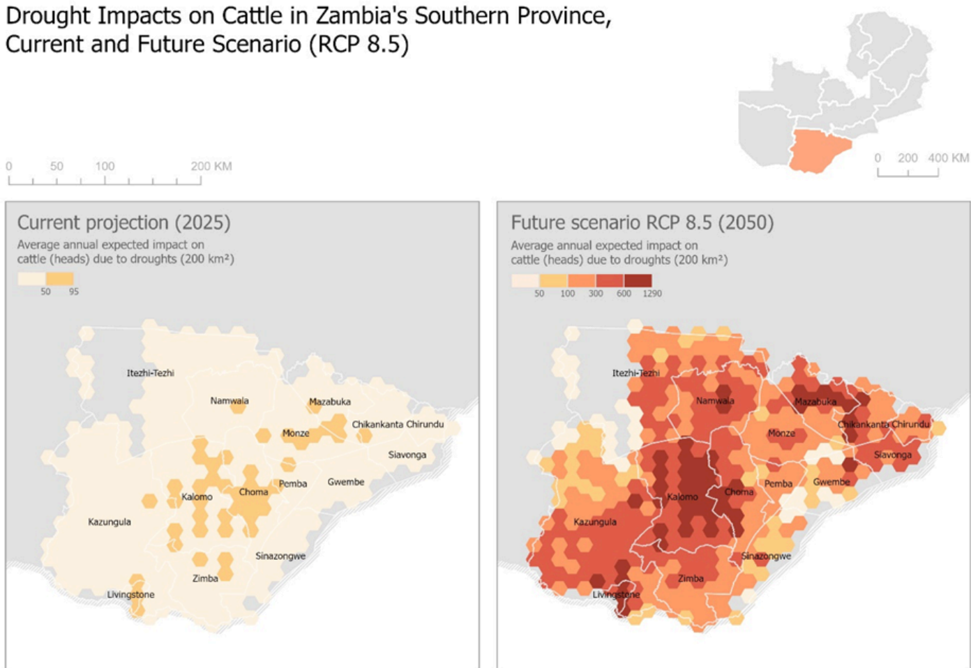
Figure 13: Drought impacts on cattle population for current and future (2050, RCP 8.5) scenarios.
