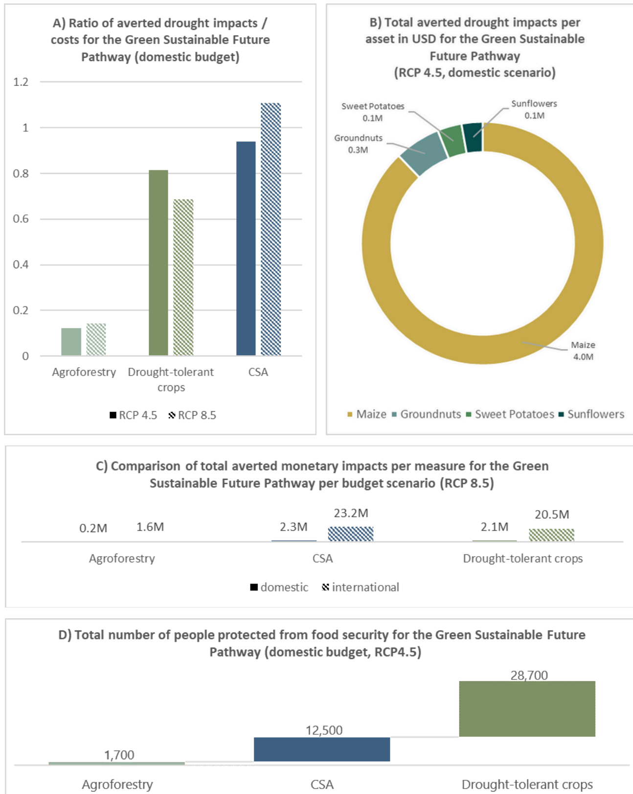
Figure 22: Key modelling outcomes of the Green Sustainable Future Pathway
