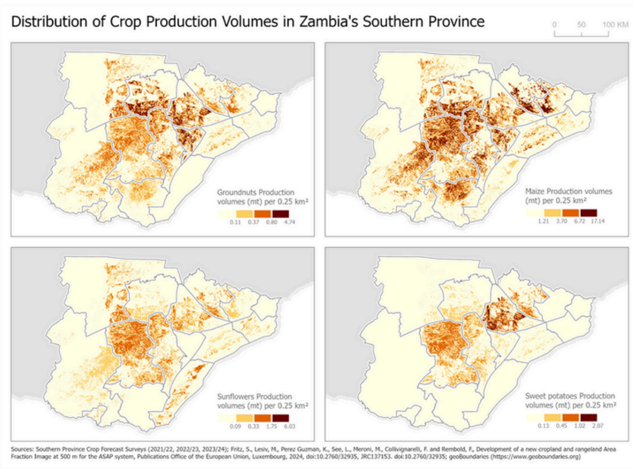
Figure 32: Distribution of key crop types
