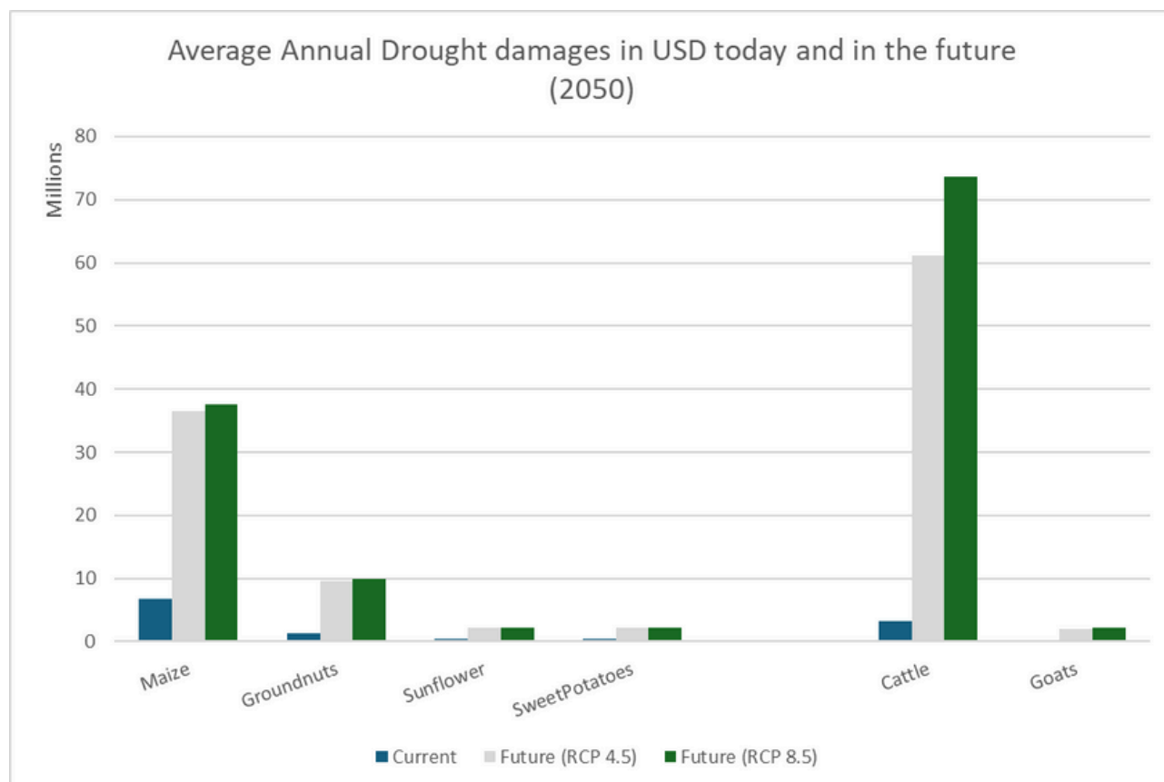
Figure 2: Average Annual Drought Damages in USD today in the future (2050).
