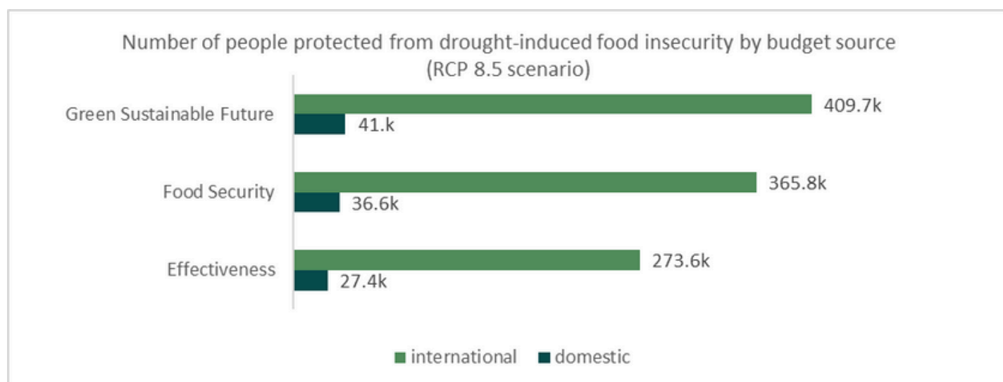
Figure 27: Total averted damages for People (RCP 8.5)
