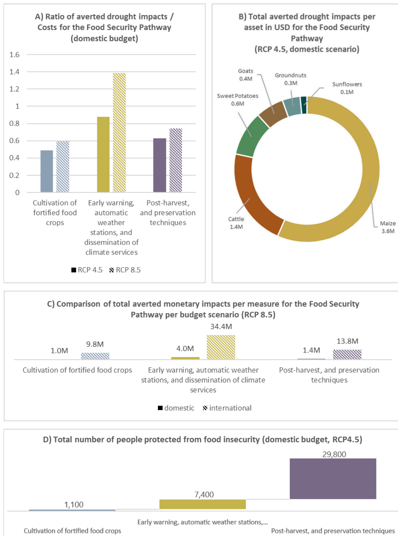
Figure 24: Key modelling outcomes of the Improving Food Security Pathway.
