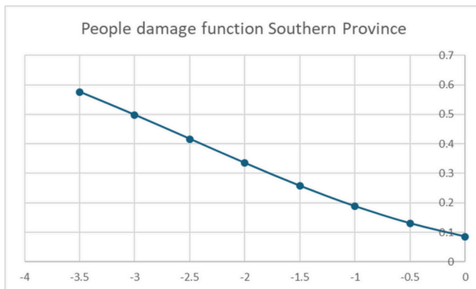
Figure 37: People damage functions, Southern Province
