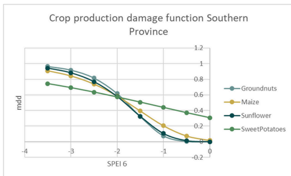
Figure 35: Crop production damage functions, Southern Province
