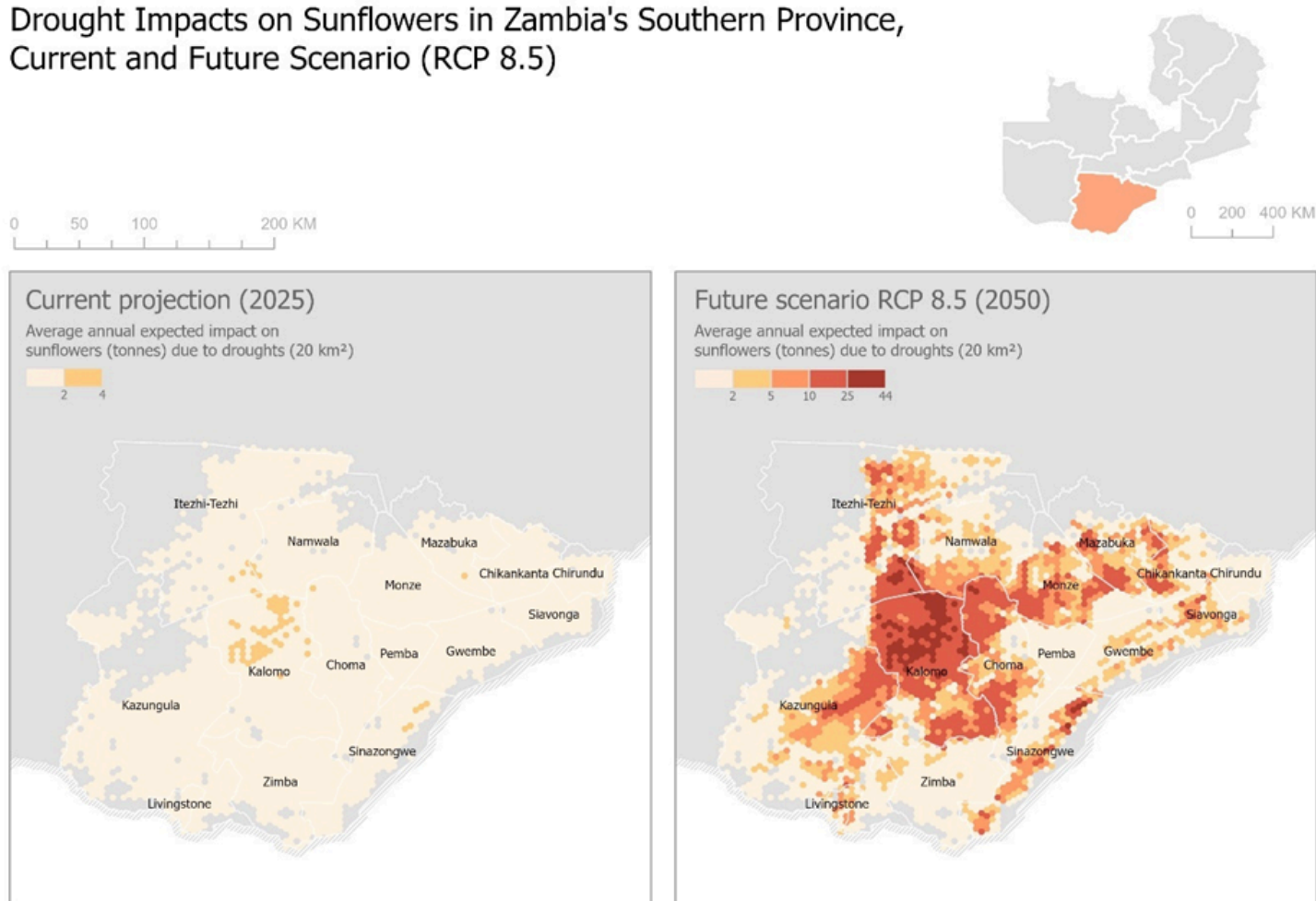
Figure 8: Drought impacts on sunflower production for current and future (2050, RCP 8.5) scenarios.
