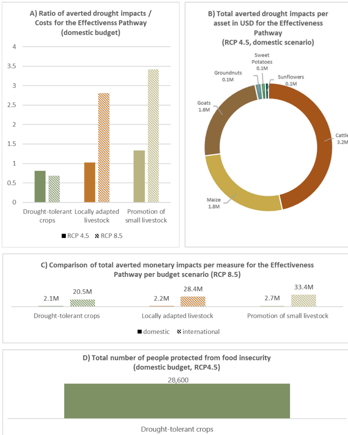
Figure 20: Key modelling outcomes of the Effectiveness Pathway
