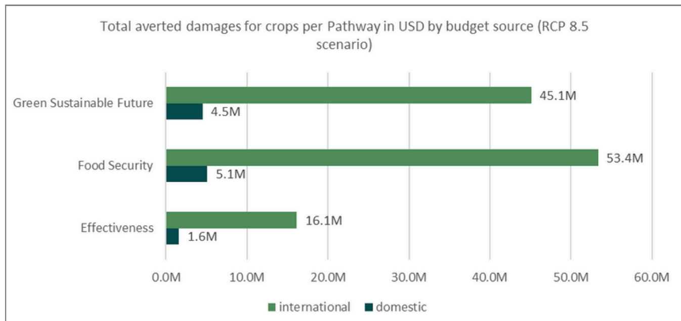
Figure 25: Total averted damages for crops (RCP 8.5)
