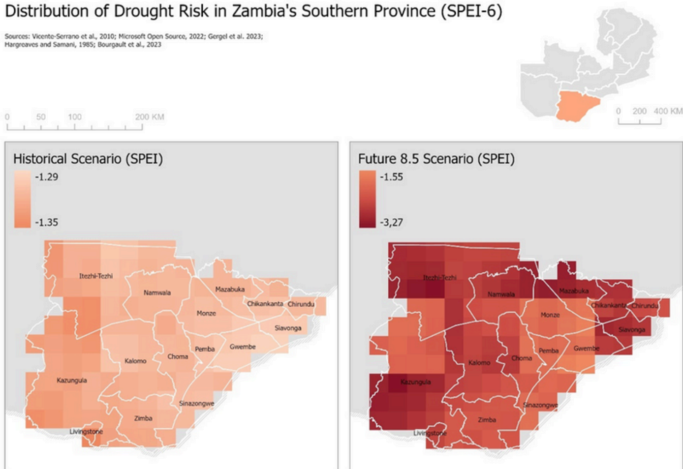
Figure 1: Distribution of Drought Risk in Zambia's Southern Province (SPEI-6).
