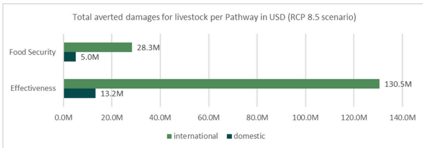
Figure 26: Total averted damages for livestock (RCP 8.5)
