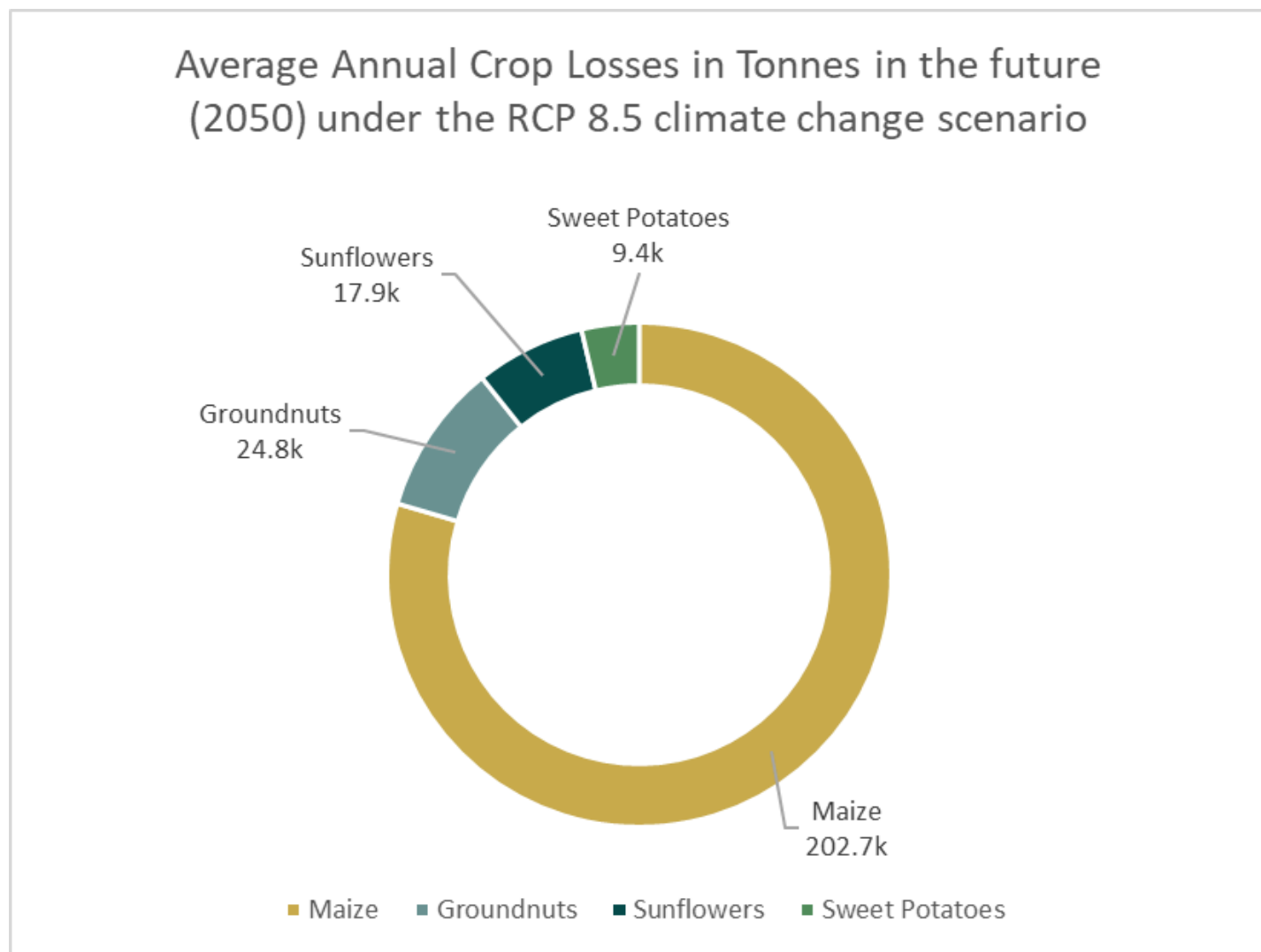
Figure 3: Average Annual Crop Losses in Tonnes in the future (2050) under the RCP 8.5 climate change scenario.
