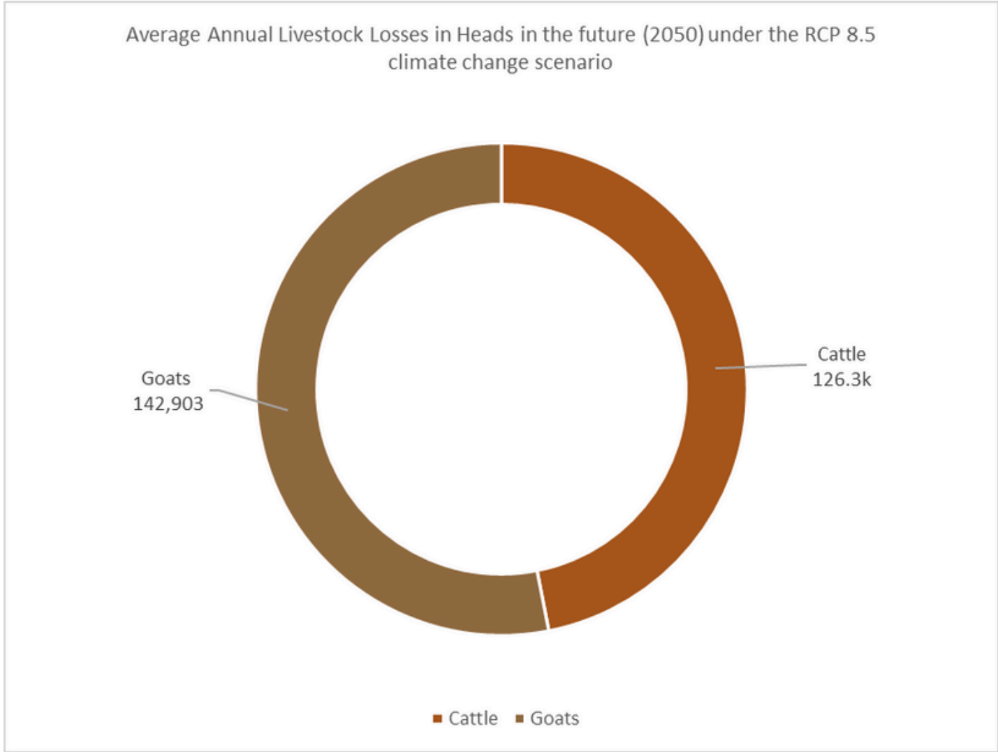
Figure 12: Average Annual Livestock Losses in Heads in the future (2050) under the RCP 8.5 climate change scenario.
